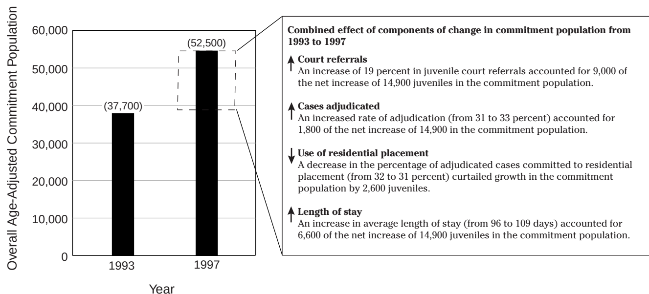
Figure 5: How much did each source of change contribute to the overall change in the population of juveniles in commitment from 1993 to 1997?
